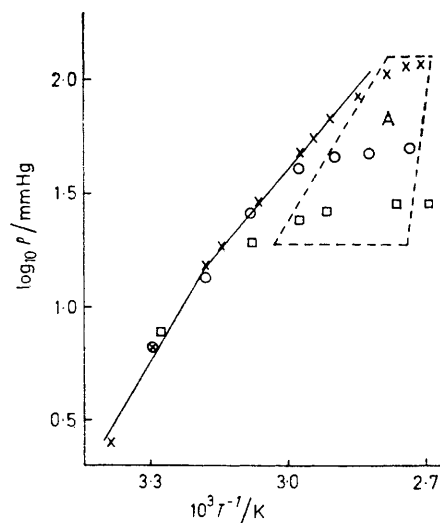
FIGURE 3 Vapour pressure data for \text{IF}_3\text{O}_2 . Points lying within frame labelled A have molecular weights within 6% of that for (\text{IF}_3\text{O}_2)_2 ; ×, ○, and □ refer to three different samples
