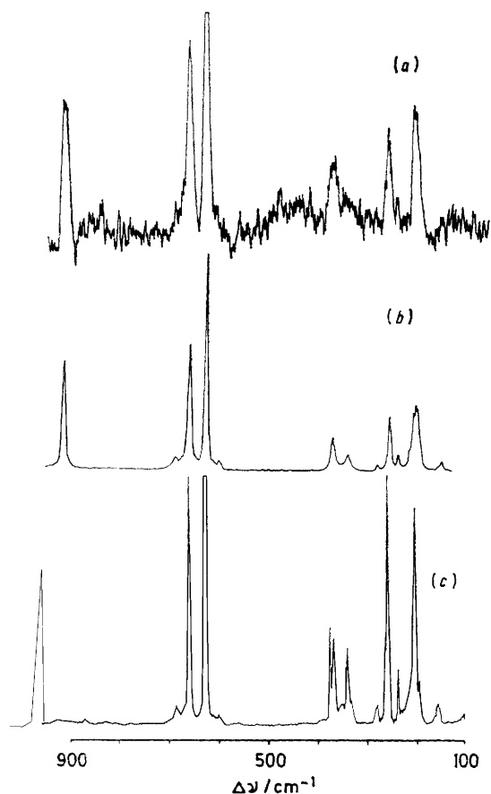
FIGURE 4 Raman spectra of \text{IF}_3\text{O}_2 (a) gas, (b), melt, and (c) solid
