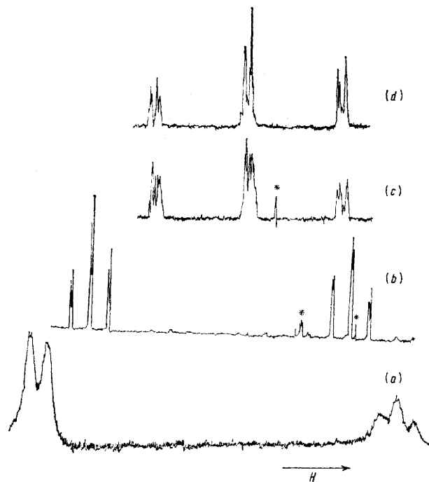
FIGURE 5 ^{19}\text{F} N.m.r. spectra at 31 °C in \text{CFC1}_3 of (a) \text{IF}_3\text{O}_2 , (b) (\text{TeF}_4\text{O})_2 , (c) high-field signal of (\text{TeF}_4\text{O})_2 on expanded scale, and (d) low-field signal of (\text{TeF}_4\text{O})_2 on expanded scale. Signals marked * are due to impurities. (For numerical values see Table 5)
