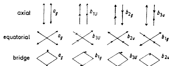
FIGURE 2 Schematic drawing of 'stretching vibrations' of (\text{TeF}_4\text{O})_2 . Motions of only terminal fluorine atoms or bridge atoms shown
